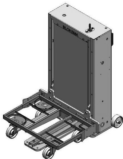
Illustrated version: semi-mobile lifter
